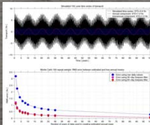
Figure 7: Upper panel – 100 year synthetic time series of Florida Current transport made up of an annual cycle, a 12 year cycle, and random noise. Lower panel – Monte Carlo style estimate of the root-mean-squared error in the predicted annual cycle signal for a day given the indicated number of years averaged together.
