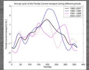
Figure 6: Annual cycle of the Florida Current transport estimated from different segments of data from the cable. (as noted in the legend).
