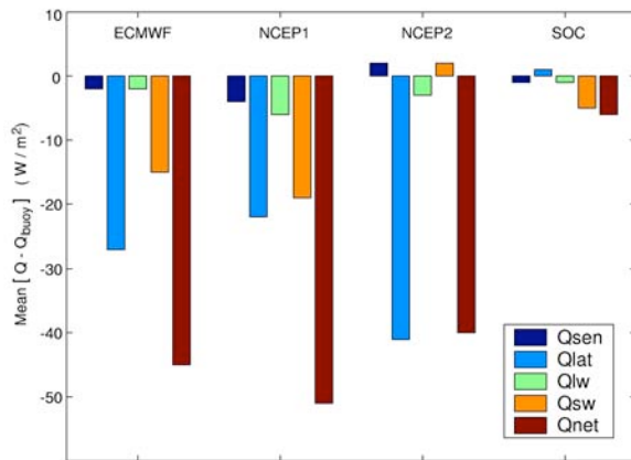
Figure 1. Differences between in-situ and modeled net heat flux at the NTAS site ( 15^{\circ} N, 51^{\circ} W) are large (4-5 times larger than the expected NTAS error of about 10 \text{ W/m}^2 ). The two-year mean net heat flux is significantly underestimated by the three models: All three models indicate a negative two-year mean net heat flux, whereas the observed value is +40 \text{ W/m}^2 . The SOC climatology and the observations agree to within the observational error.
