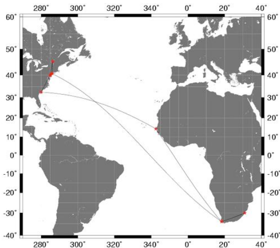
Figure 2. The route of the SeaLand Express. The VOS AUTO-IMET system was installed in March 2004. The ship is on a cross-equatorial route between the U.S. east coast and South Africa takes about 7 weeks to complete. It includes a high density XBT run from Cape Town to New York (AX-8).
