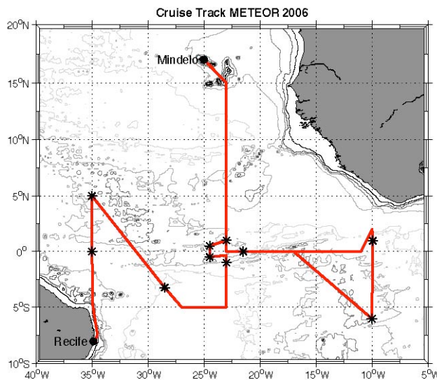
Figure.: Cruise track of METEOR M68/2 in June 2006. Stars represent mooring positions. Mooring at 35°W, 0°N and 5 moorings near 23°W, 0°N are current meter moorings, other moorings are sound source moorings for a RAFOS float project that will be completed in 2006.
