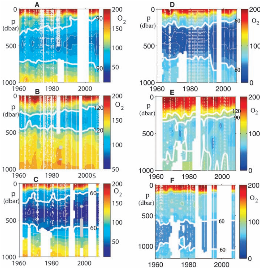
Fig. 2. Dissolved oxygen concentration ( \mu\text{mol kg}^{-1} shown in color maps (20, 21) versus time (1960–2008) and pressure (1 dbar \sim 1 m) with sample locations (white dots). (A) The eastern tropical North Atlantic ( 10^\circ to 14^\circ\text{N} , 20^\circ to 30^\circ\text{W} ), contoured at 90 \mu\text{mol kg}^{-1} (thick white line). (B) The central equatorial Atlantic ( 3^\circ\text{S} to 3^\circ\text{N} , 28^\circ to 18^\circ\text{W} ), contoured at 120 \mu\text{mol kg}^{-1} (thick white line). (C) The eastern tropical South Atlantic at ( 14^\circ to 8^\circ\text{S} , 4^\circ to 12^\circ\text{E} ), contoured at 60 \mu\text{mol kg}^{-1} (thick white line). (D) The eastern equatorial Pacific Ocean ( 5^\circ\text{S} to 5^\circ\text{N} , 105^\circ to 115^\circ\text{W} ), contoured at 60 \mu\text{mol kg}^{-1} (thick white line). (E) The central equatorial Pacific Ocean ( 5^\circ\text{S} to 5^\circ\text{N} , 165^\circ to 175^\circ\text{W} ), contoured at 90 and 120 \mu\text{mol kg}^{-1} (thick white lines). (F) The eastern equatorial Indian Ocean ( 5^\circ\text{S} to 0^\circ , 90^\circ to 98^\circ\text{E} ), contoured at 60 \mu\text{mol kg}^{-1} (thick white line).
