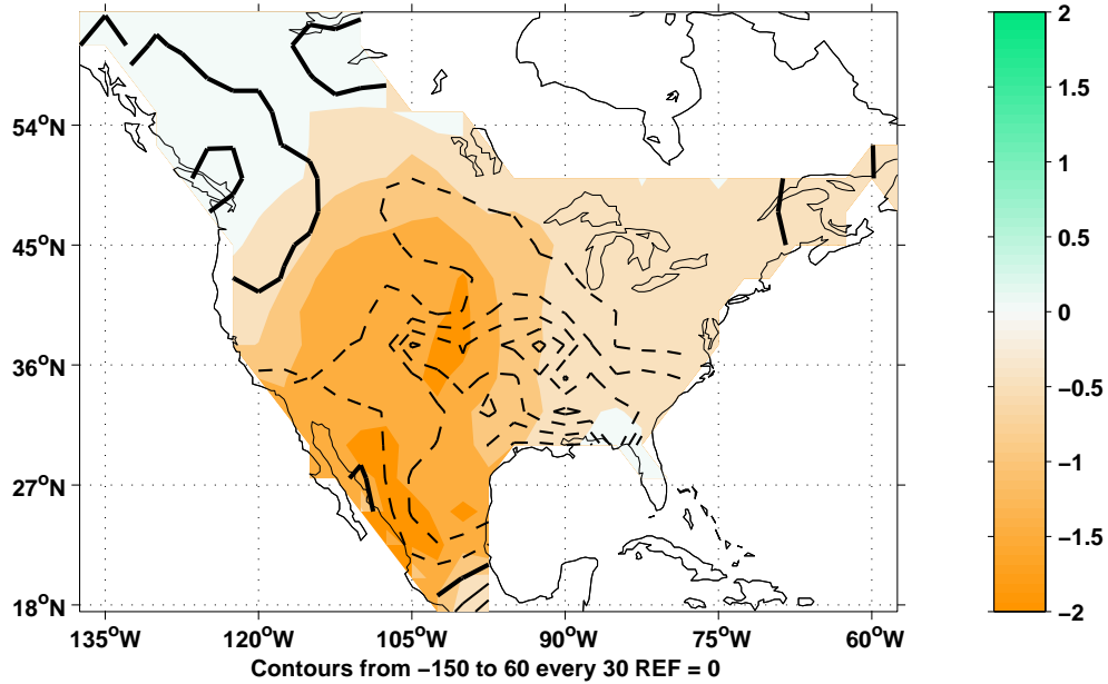
Filtered PDSI Anom V2a(colors) and GOGA Soil Moisture Anom (contours), Mode 1 94%
