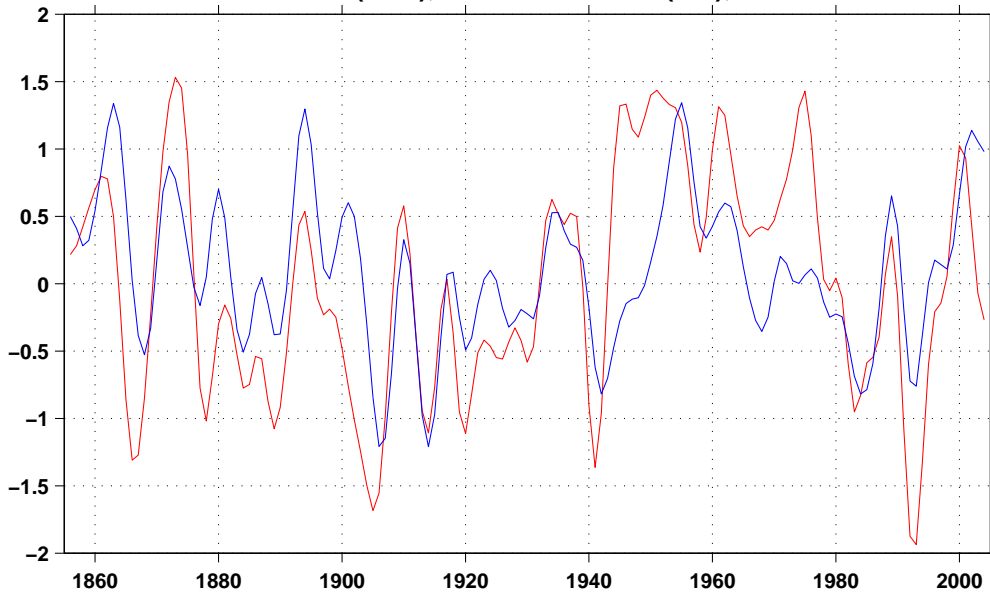
PDSI Anom (blue), GOGA SM Anom (red), Corr 0.58
