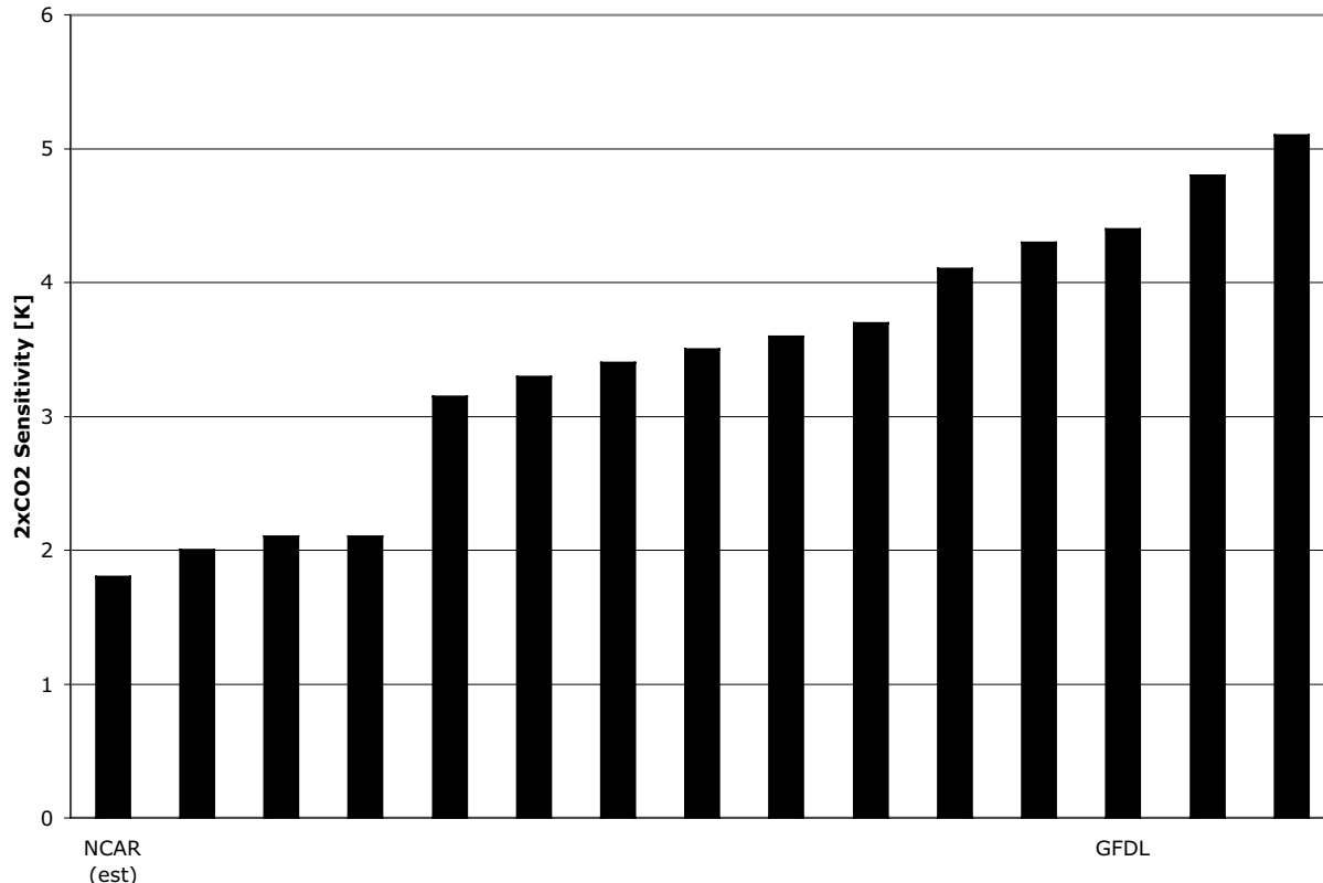
Figure 1. Climate model sensitivity (change of global mean temperature) for a range of climate models for a prescribed doubling of CO 2 . Note the especially large spread between the GFDL and NCAR-CCSM models.
